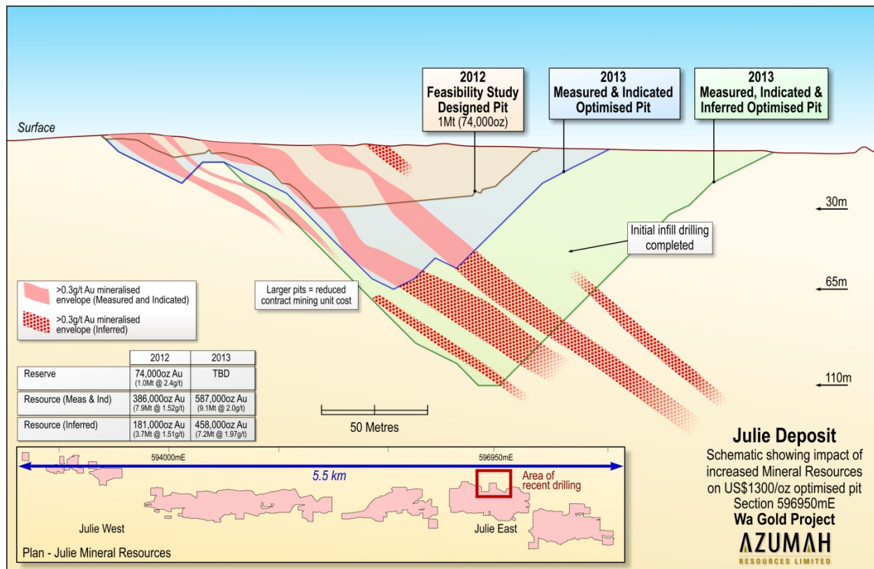
Figure 1: Impact of increased Mineral Resources and higher grade on Julie optimised pits
