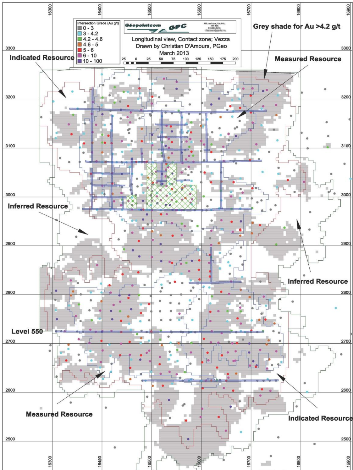
Veza Longitudinal Section with Resources classification using 4.2 g/t Au cut-off for Measured and Indicated Resources, and 3 g/t Au cut-off for Inferred Resources.
