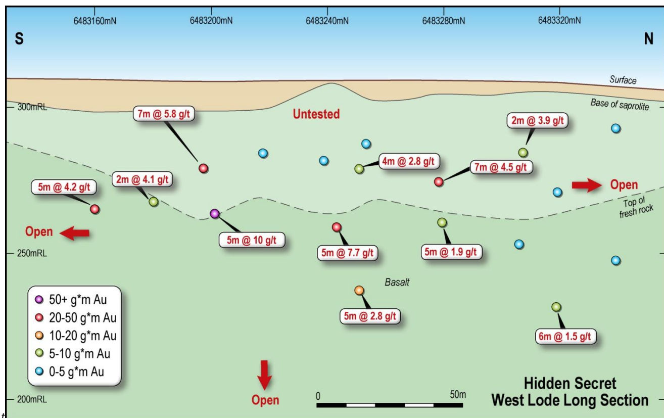
Figure 5: Long Section of the Western Lode at Hidden Secret, Eundynie Project, Higginsville. Estimate true widths are 90% of downhole widths.
