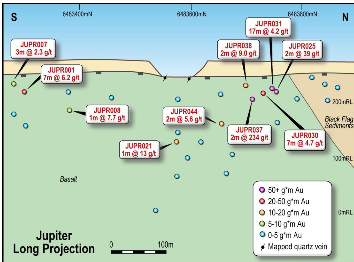
Figure 4: Long Section of the Jupiter Prospect at the Challenge Project, Higginsville. Estimate true widths are 60-70% of downhole widths.
