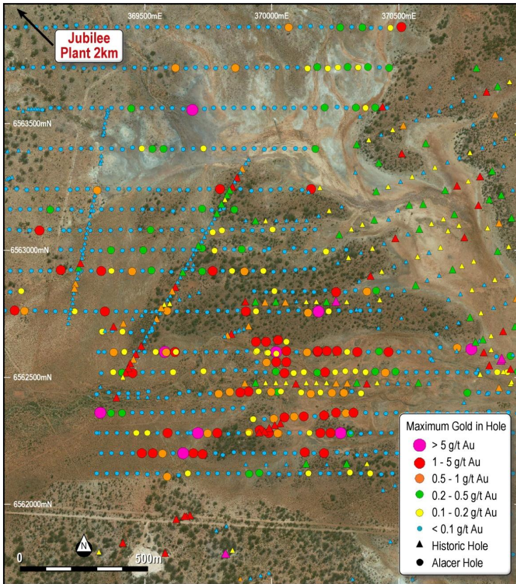
Figure 2: Wedge Prospect at Location 48. Widespread gold anomalism is seen in broad early stage aircore drilling. Alacer drilling is represented as circles and effective historical drilling as triangles. Drill collars color coded to maximum gold assay value in (red > 1.0g/t gold).
