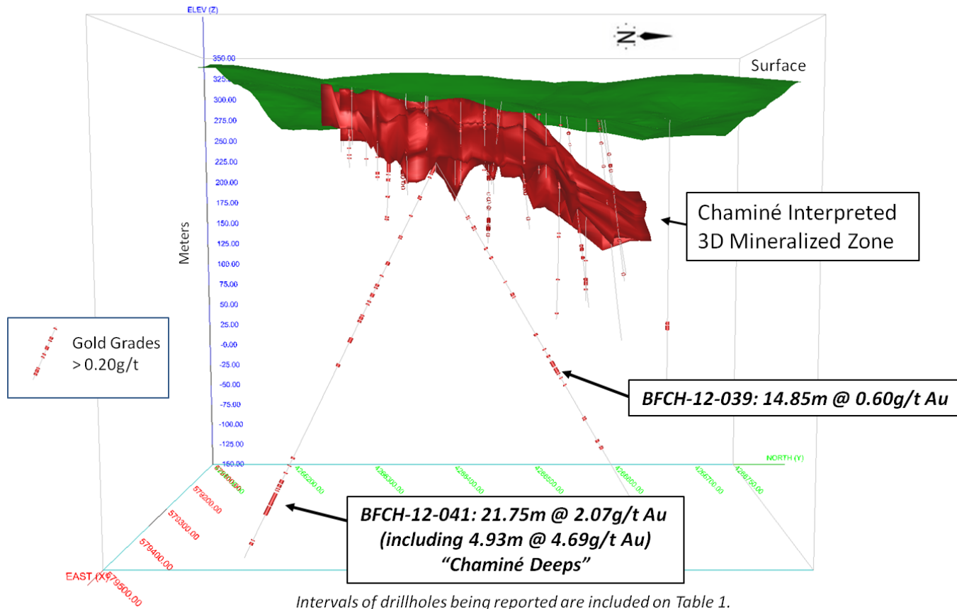
Figure 2: 3D view of the Chaminé deposit including results of the first 2 deep drillholes and including drill traces of all Colt drillholes reported to date.
